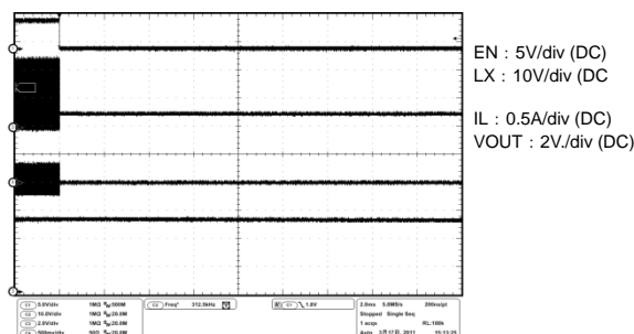
Figure 30. Stop Waveform
