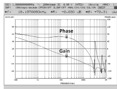
Figure 26. Frequency Response Characteristics (Io=3.0A)
